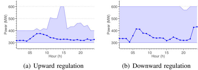
Fig. 1: Hourly minimum, average, and maximum capacity procurements for upward and downward regulation in California. The plots are based on historic data of CAISO in 2012.
